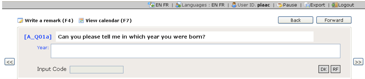
Figure 7.3: Screenshot of a numeric entry to which is associated a range constraint and a consistency check
