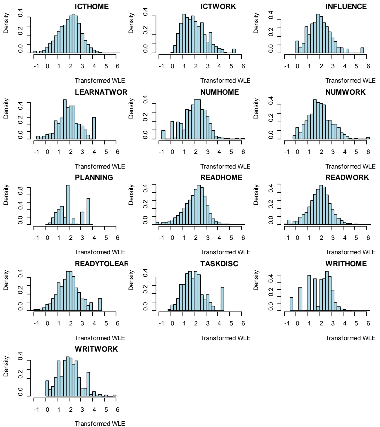
Figure 20.3: WLE distributions
