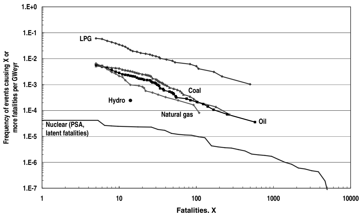
Figure 4.12 Comparison of frequency-consequence curves for full energy chains in OECD countries for the period 1969-2000
