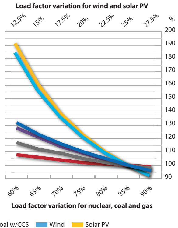
Figure 6.22: LCOE as a function of a variation in the load factor (at 10% discount rate)
