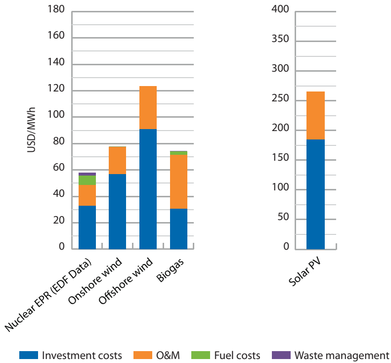
Figure 4.5a: France – levelised costs of electricity (at 5% discount rate)
