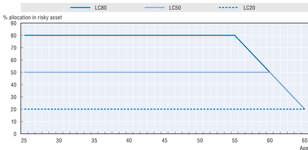
Figure 5.3. Shapes of the different life cycle investment strategies analysed (LC80, LC50, LC20)
