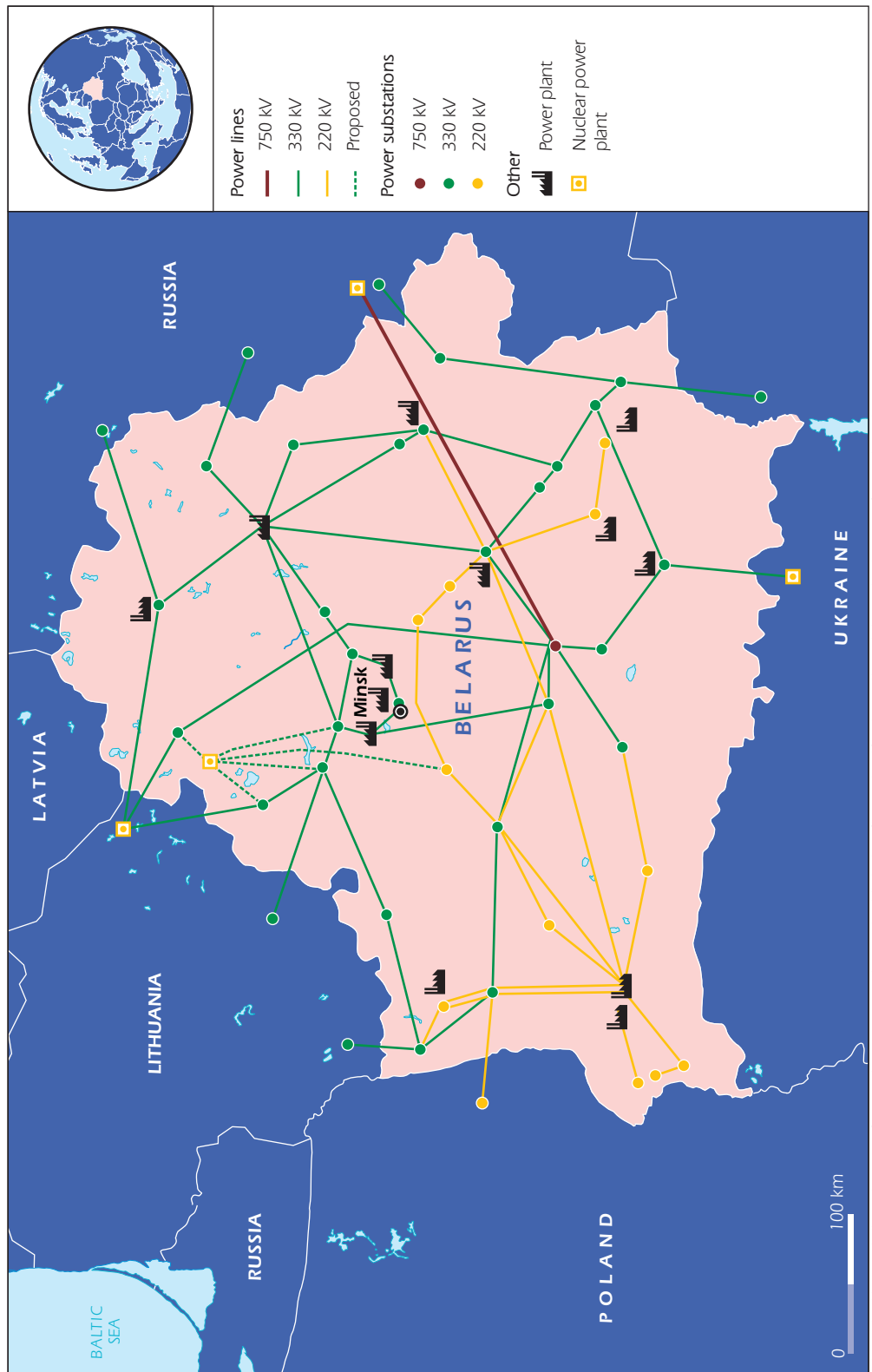
Figure 3.2.1 Electricity network, Belarus
