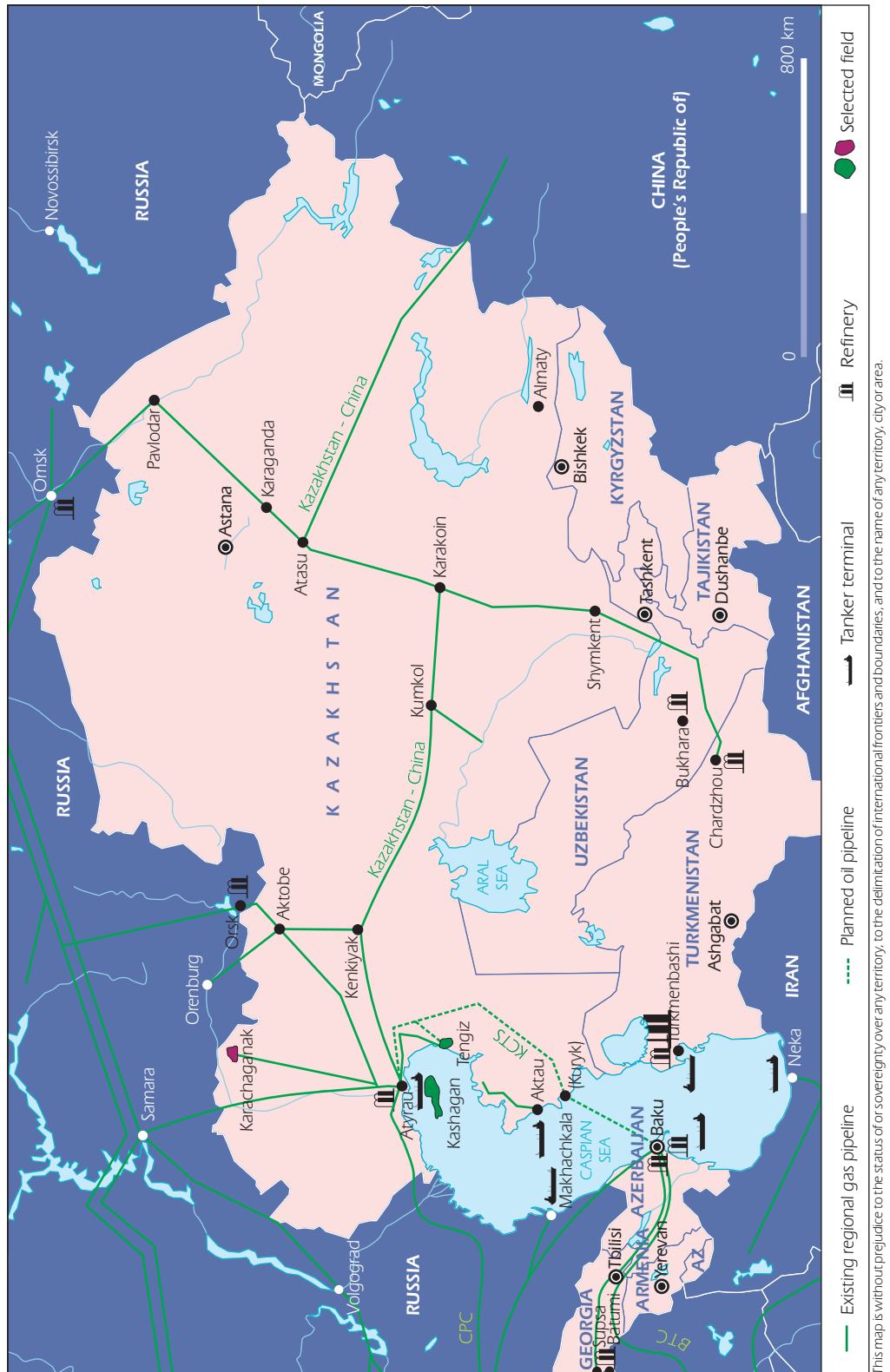
Figure 5.2.2 Central Asia oil pipeline network
