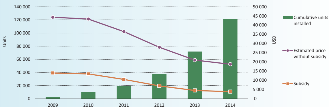
Figure 8: Ene-Farm fuel cell micro co-generation cumulative sales, subsidies and estimated prices, 2009-14
