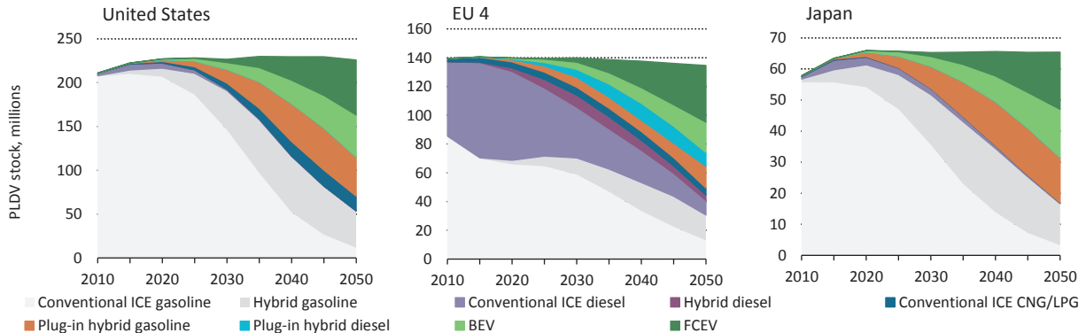
Figure 13: PLDV stock by technology for the United States, EU 4 and Japan in the 2DS high H 2
