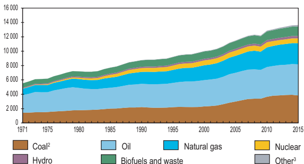
World 1 TPES from 1971 to 2015 by fuel (Mtoe)
