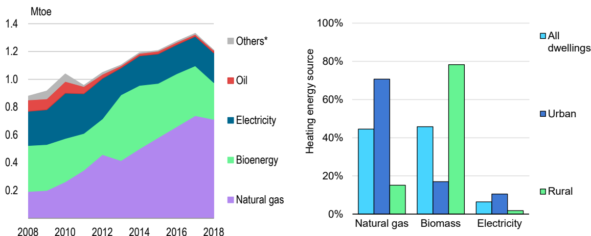
Figure 2 TFC in Georgia's residential sector (left) and heating fuel by location (right)
