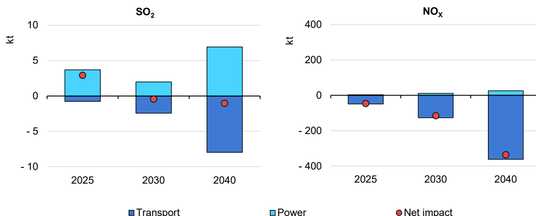
Figure 3.5 Avoided and indirect \text{SO}_2 and \text{NO}_x emissions through EVs in the Stated Policies Scenario, 2025-2040
