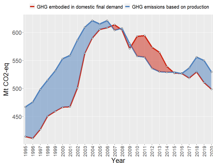
Figure 8. Australia - production-based and demand-based greenhouse gas (GHG) emissions 1995 to 2020, Million tonnes of CO 2 equivalent (Mt CO 2 -eq)
