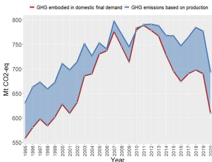
Figure 8. Canada - production-based and demand-based greenhouse gas (GHG) emissions 1995 to 2020, Million tonnes of CO 2 equivalent (Mt CO 2 -eq)
