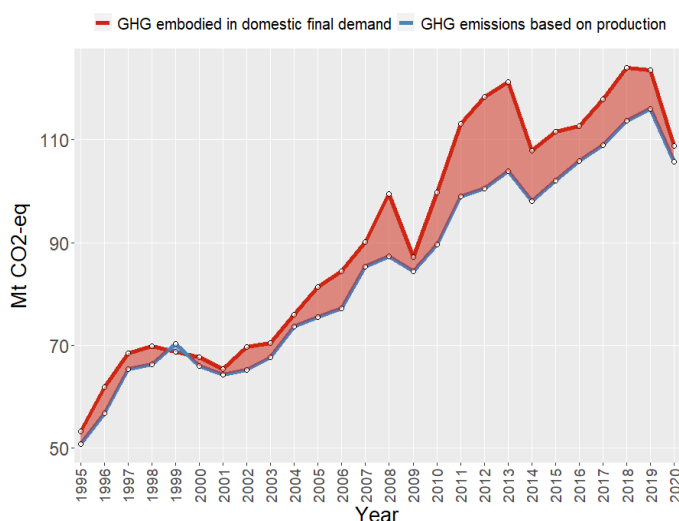
Figure 8. Chile - production-based and demand-based greenhouse gas (GHG) emissions 1995 to 2020, Million tonnes of CO 2 equivalent (Mt CO 2 -eq)
