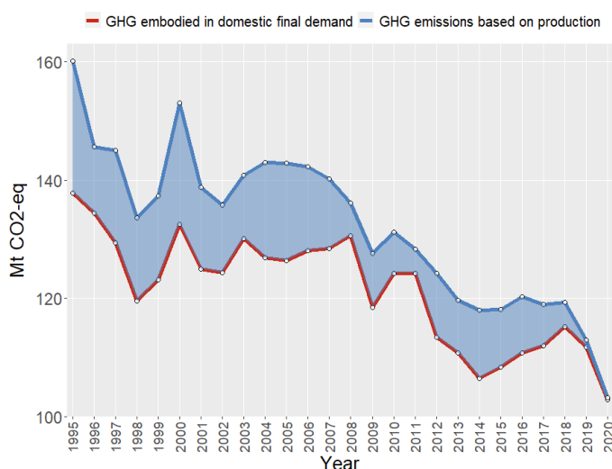
Figure 8. Czechia - production-based and demand-based greenhouse gas (GHG) emissions 1995 to 2020, Million tonnes of CO 2 equivalent (Mt CO 2 -eq)
