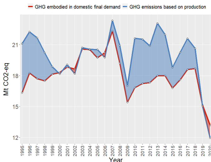
Figure 8. Estonia - production-based and demand-based greenhouse gas (GHG) emissions 1995 to 2020, Million tonnes of CO 2 equivalent (Mt CO 2 -eq)
