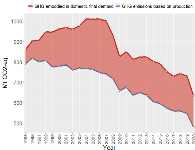
Figure 8. United Kingdom - production-based and demand-based greenhouse gas (GHG) emissions 1995 to 2020, Million tonnes of CO 2 equivalent (Mt CO 2 -eq)
