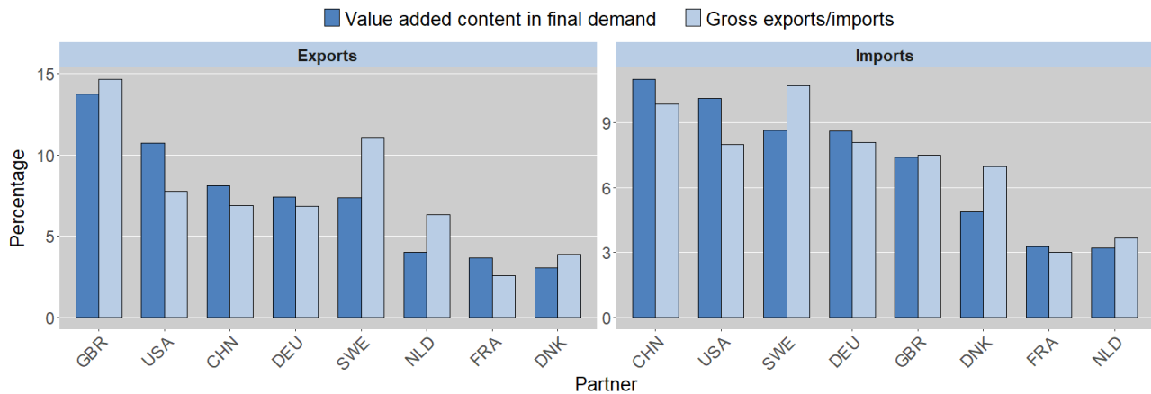
Figure 5. Norway - main trade partners As a percentage of total gross and value-added exports and imports, 2020
