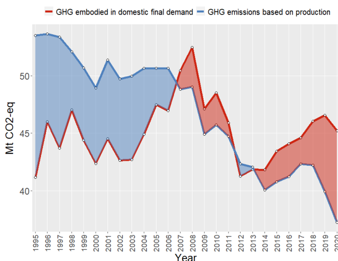
Figure 8. Slovak Republic - production-based and demand-based greenhouse gas (GHG) emissions 1995 to 2020, Million tonnes of CO 2 equivalent (Mt CO 2 -eq)
