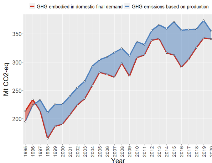
Figure 8. Thailand - production-based and demand-based greenhouse gas (GHG) emissions 1995 to 2020, Million tonnes of CO 2 equivalent (Mt CO 2 -eq)
