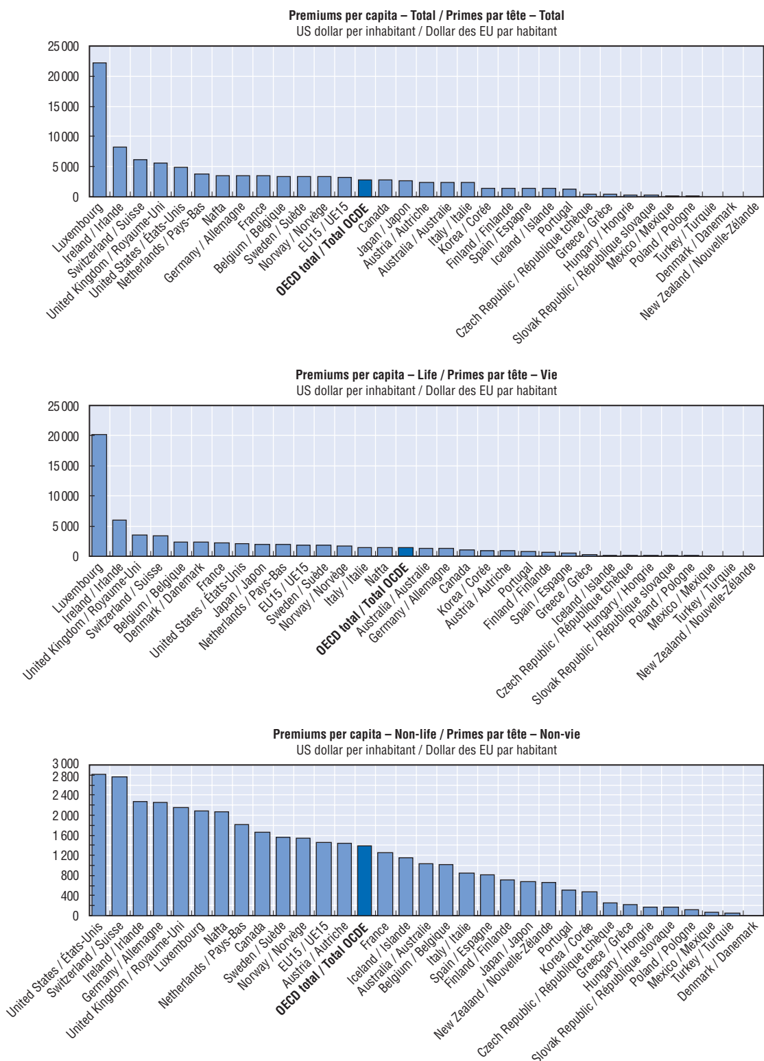
Figure I.4. Density, 2004 / Densité, 2004 Direct gross premiums/Population / Primes brutes directes/Population
