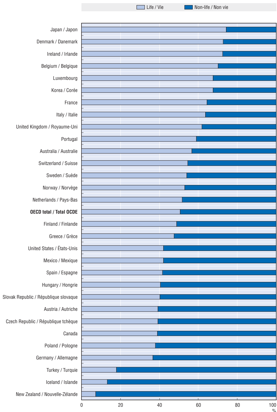
Figure I.2. Life and non-life insurance, 2004 / Part de l'assurance-vie et non-vie, 2004
