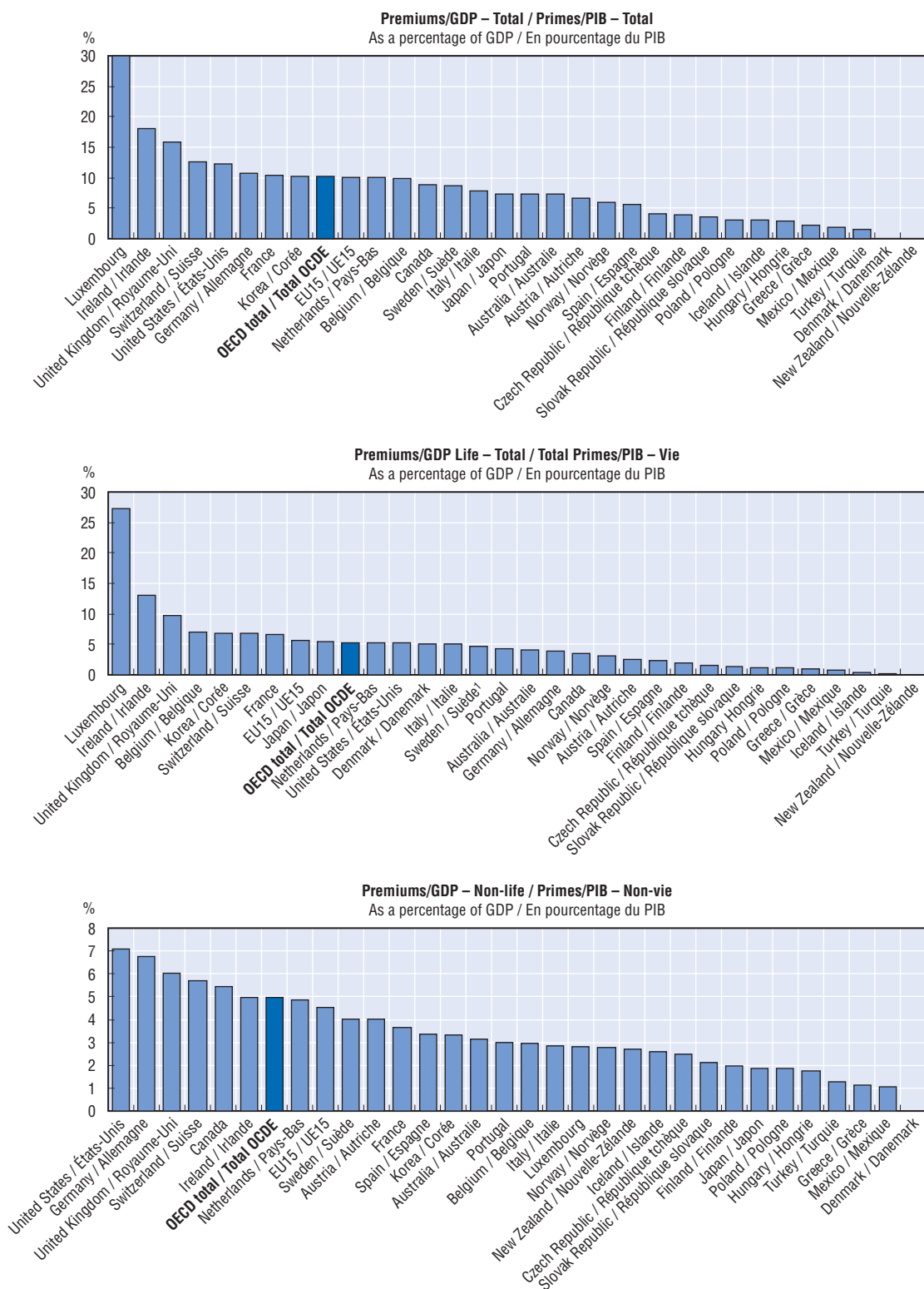
Figure I.3. Penetration, 2004 / Pénétration, 2004 Direct gross premiums – GDP / Primes brutes directes – PIB
